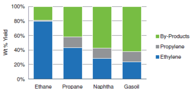
Product Yield by Feedstock
