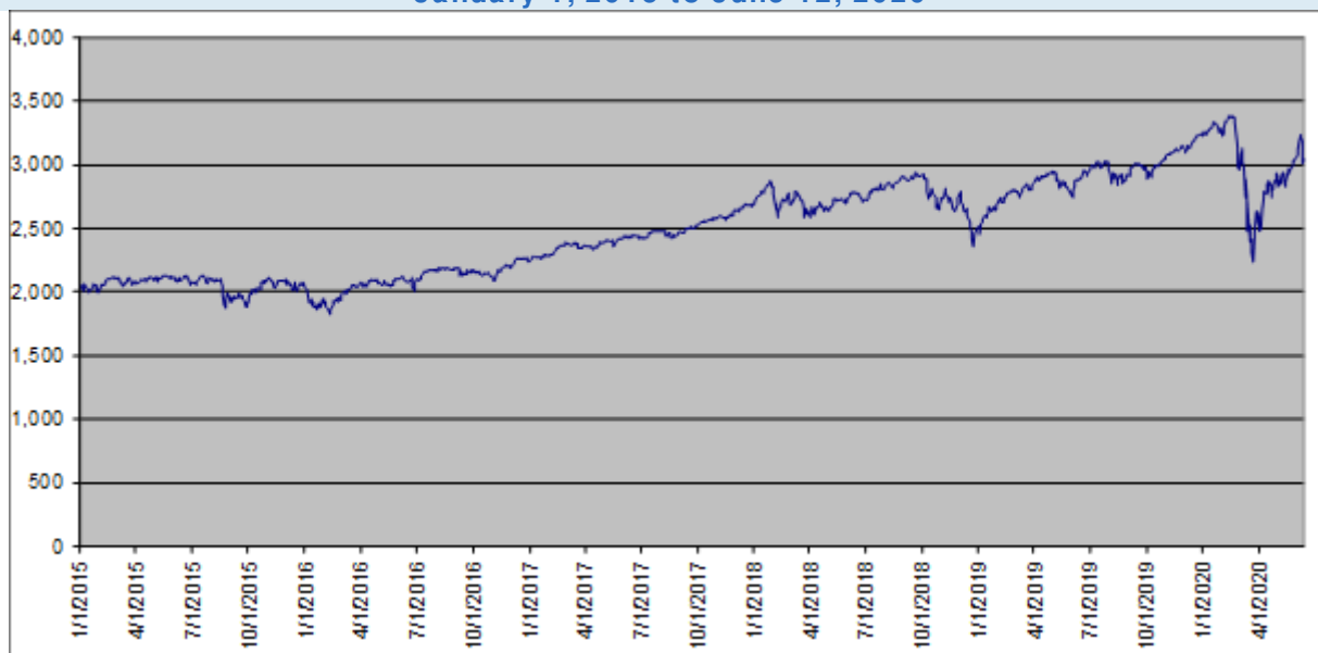
SPX Index Daily Closing Values January 1, 2015 to June 12, 2020
