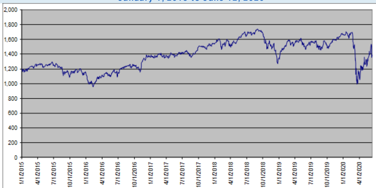
RTY Index Daily Closing Values January 1, 2015 to June 12, 2020
