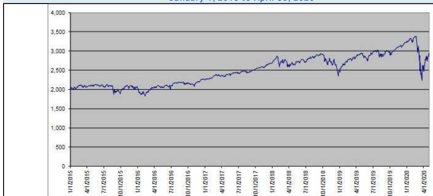
S&P 500® Index Daily Index Closing Values January 1, 2015 to April 30, 2020
