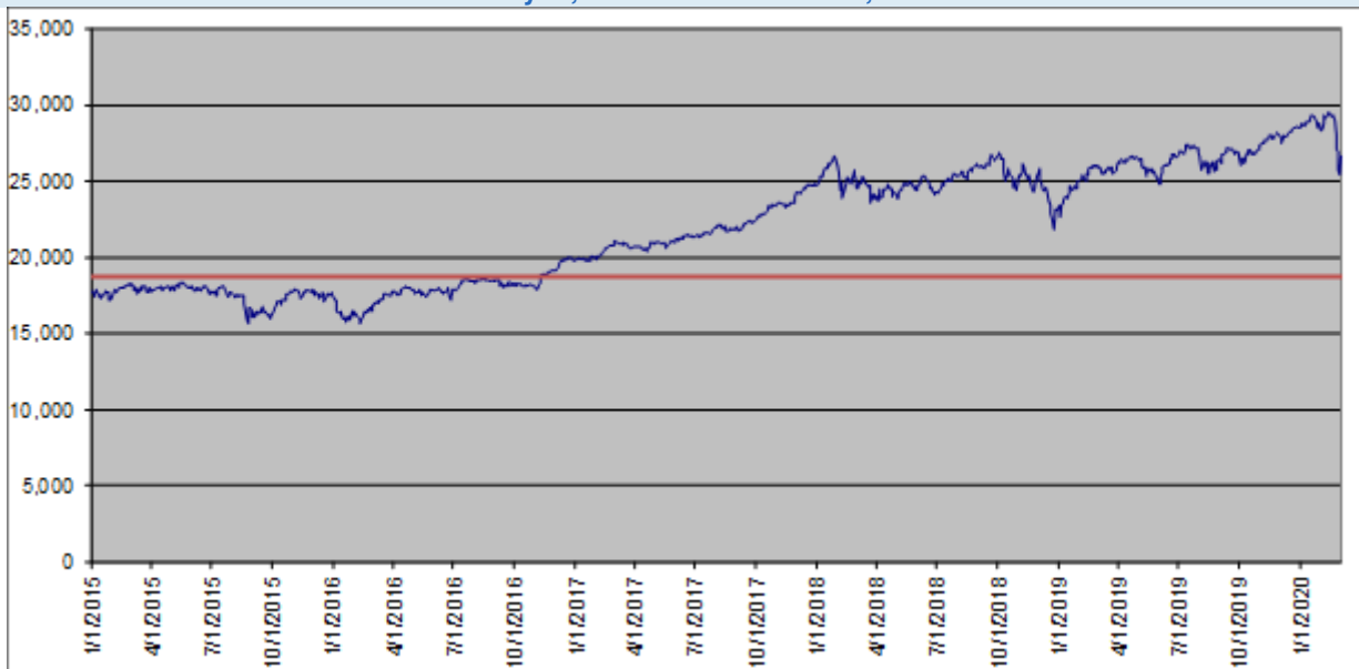
INDU Index Daily Closing Values January 1, 2015 to March 31, 2020
