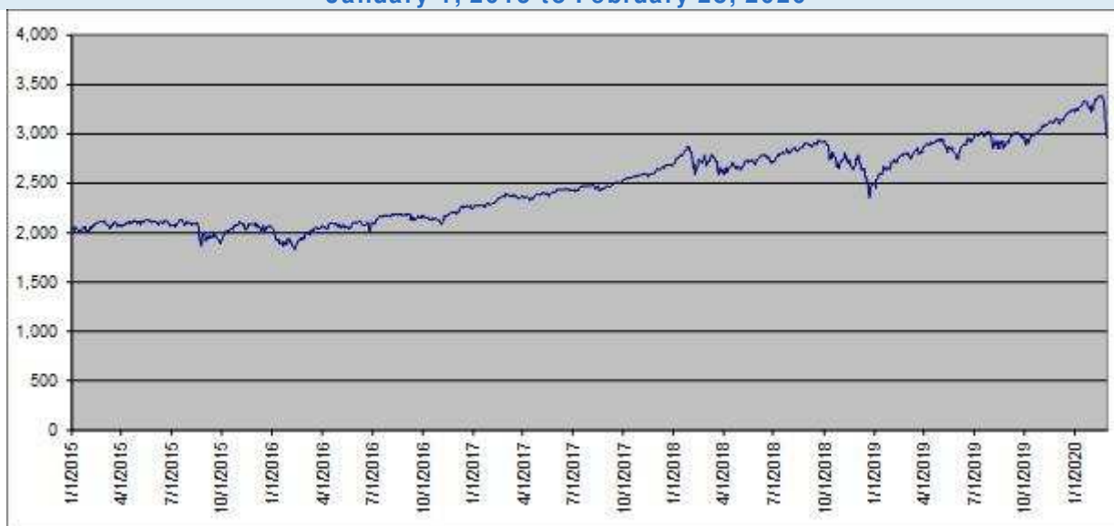
SPX Index Daily Closing Values January 1, 2015 to February 28, 2020
