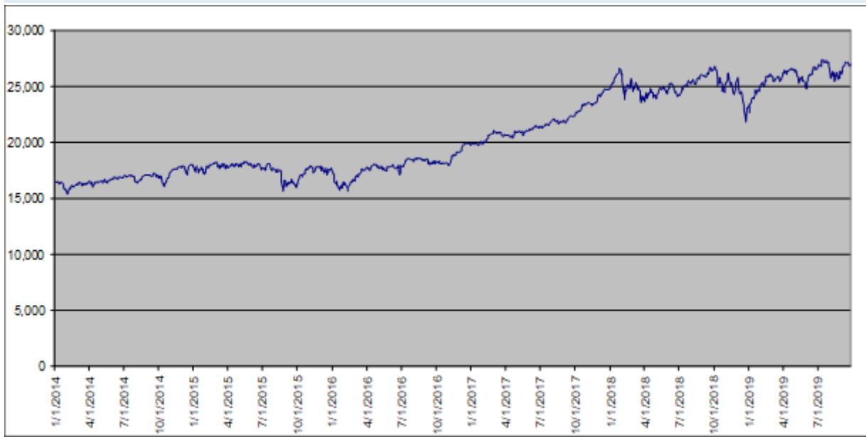
INDU Index Daily Closing Values January 1, 2014 to September 25, 2019
