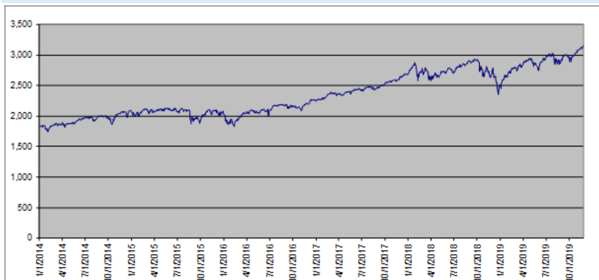
SPX Index Daily Closing Values January 1, 2014 to November 27, 2019
