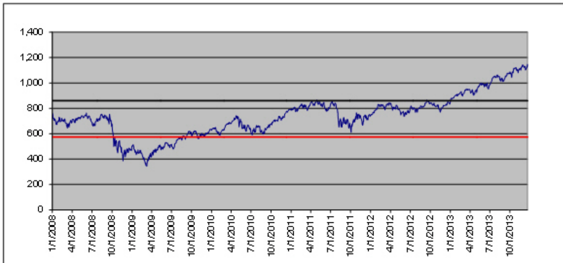
RTY Index Daily Closing Values January 1, 2008 to December 20, 2013
