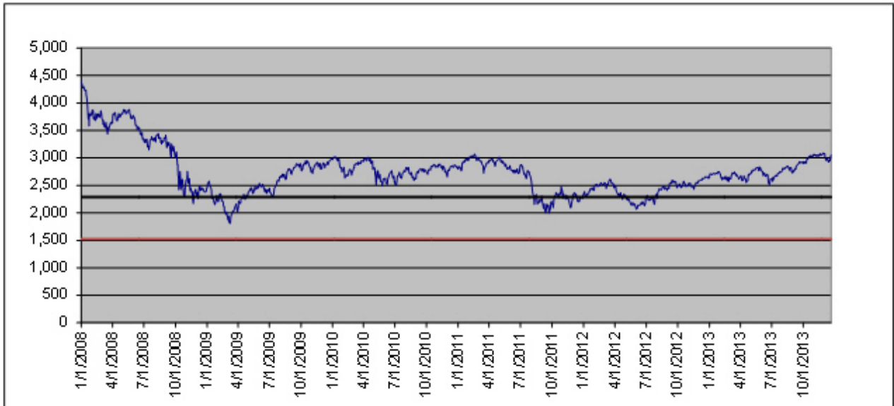
SX5E Index Daily Closing Values January 1, 2008 to December 20, 2013
