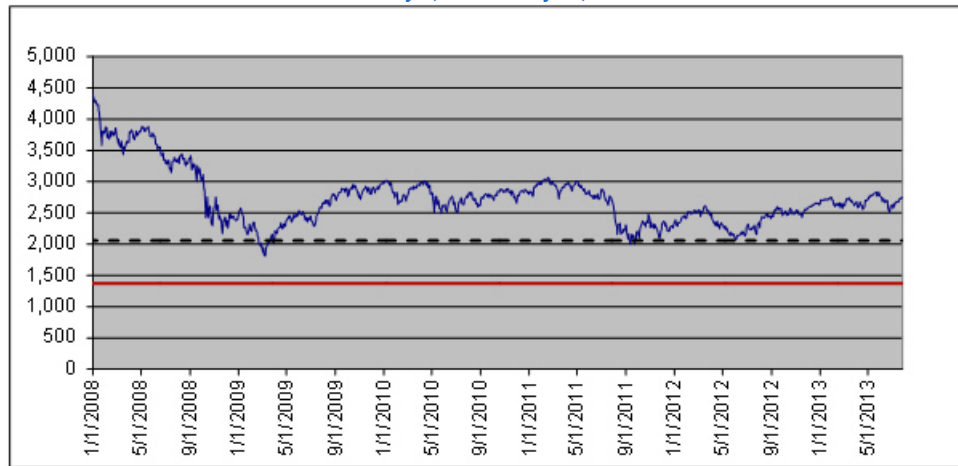
SX5E Index Daily Closing Values January 1, 2008 to July 26, 2013
