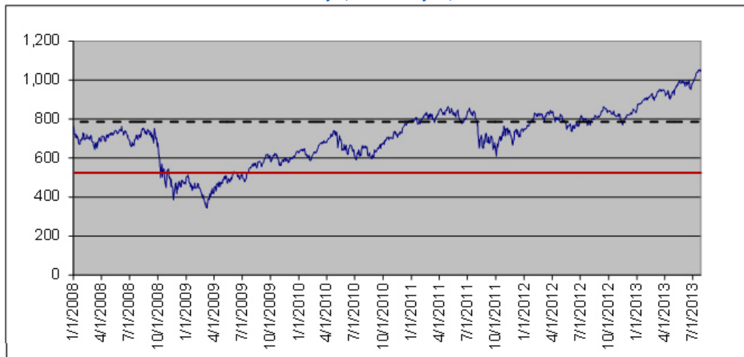
RTY Index Daily Closing Values January 1, 2008 to July 26, 2013
