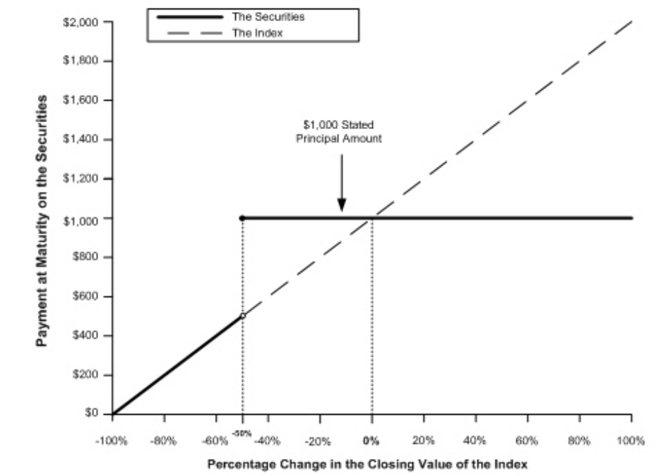
Payoff Diagram
