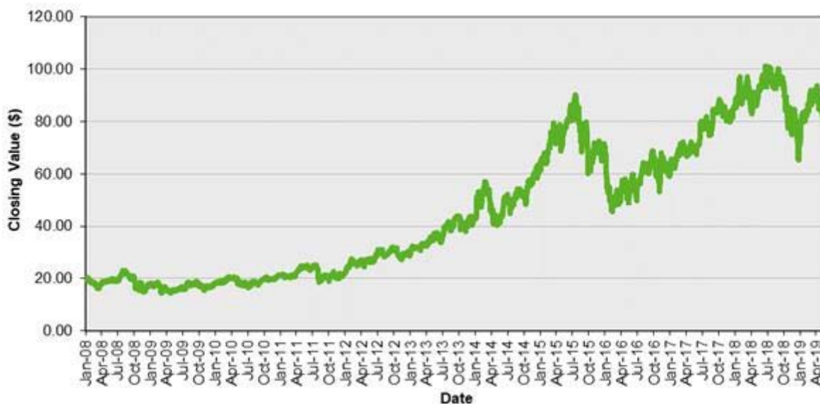
SPDR® S&P® Biotech ETF – Historical Closing Values January 2, 2008 to May 24, 2019
