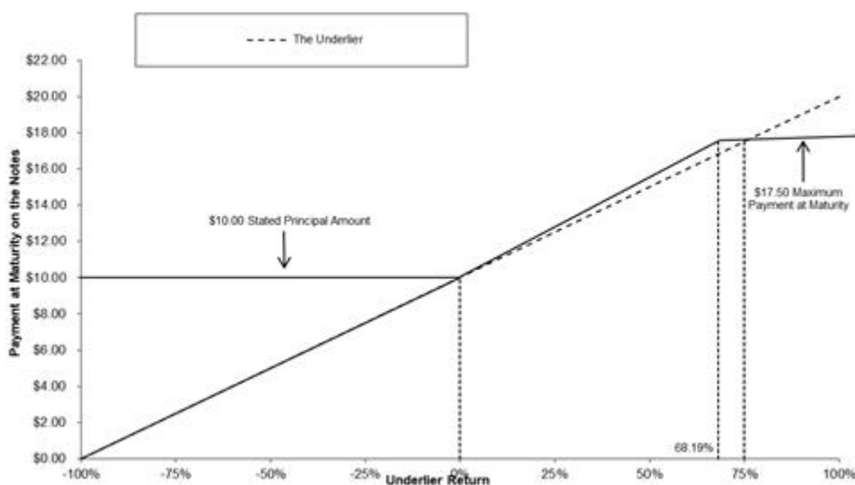
Payoff Diagram
