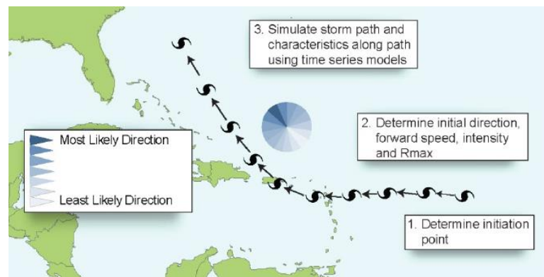
Figure 3: Storm Track Generation (1)
