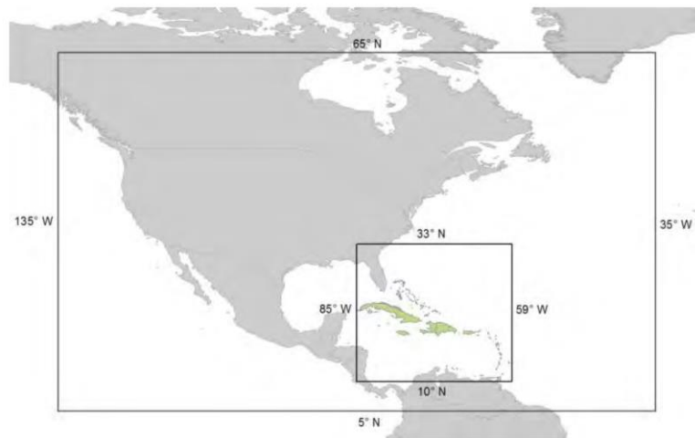
Figure 1: Caribbean Model Domain (1)
