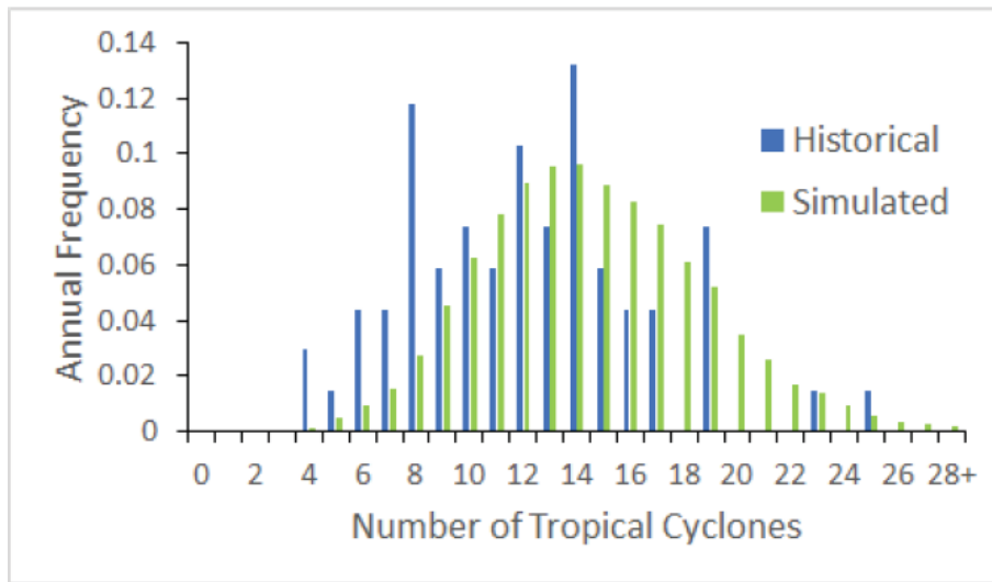
Figure 4: Comparison of Historical versus Simulated Annual Landfall Frequency (1)
