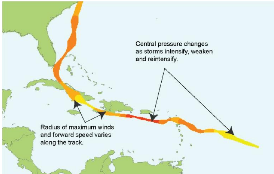
Figure 2: Tropical Cyclone Parameters Along a Storm Track (1)
