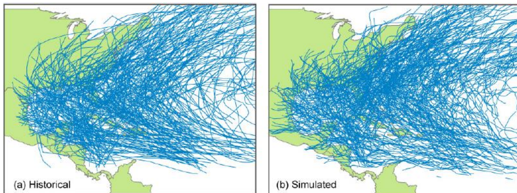
Figure 5: Comparison of Historical versus Simulated Storm Tracks for the Atlantic Basin (1)
