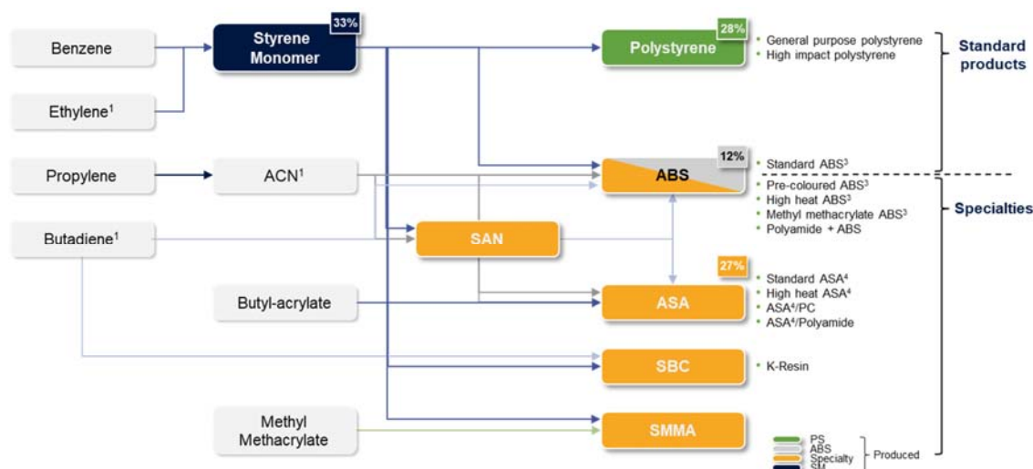
Product scope in the styrenics value chain
